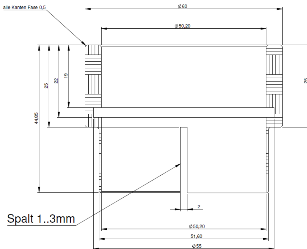
picture 2: dimensions in mm
