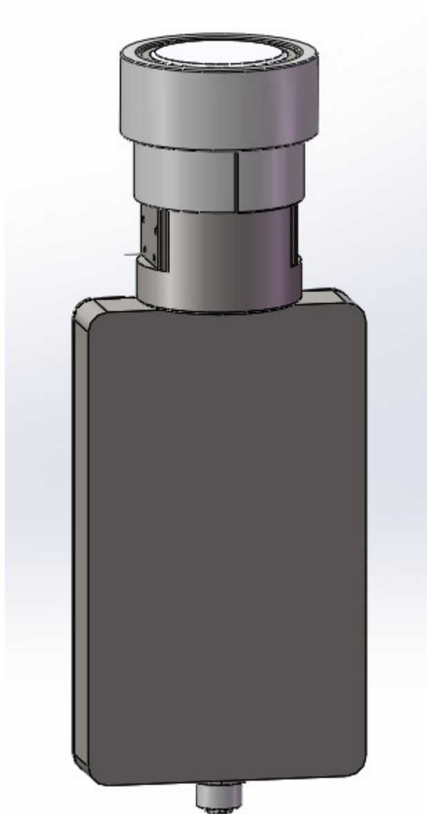
picture 3: Adapter with microwave sensor ( The clamp over the slotted part of the adapter is not shown.)
